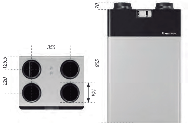
VMC VEX 250 / 350
