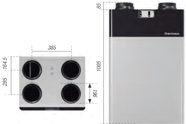
VMC VEX 500
